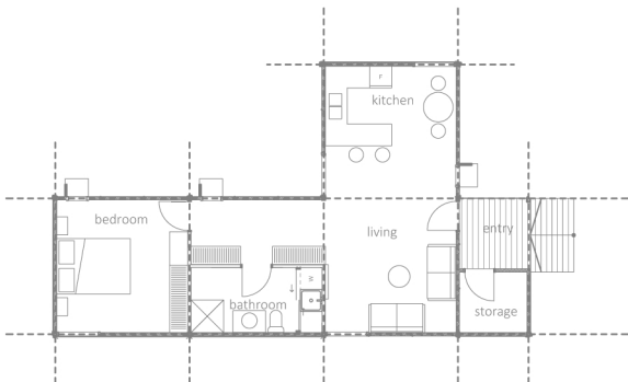
floor plan__version two 60.9 m 2
